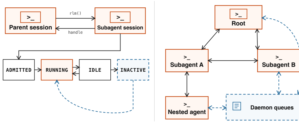
Figure 3: Multi-agent orchestration lifecycle and direct agent-to-agent communication.
